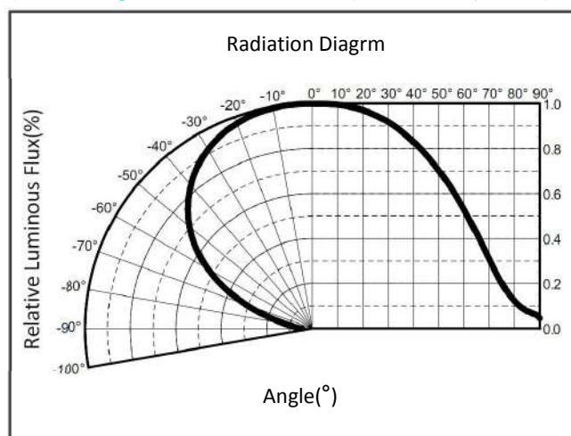
f) Beam Angle Characteristics 光束角 ( I_f = 700\text{ mA} , T_j = 25^\circ\text{C} )
